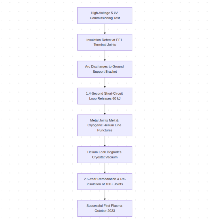
2021 JT-60SA incident
